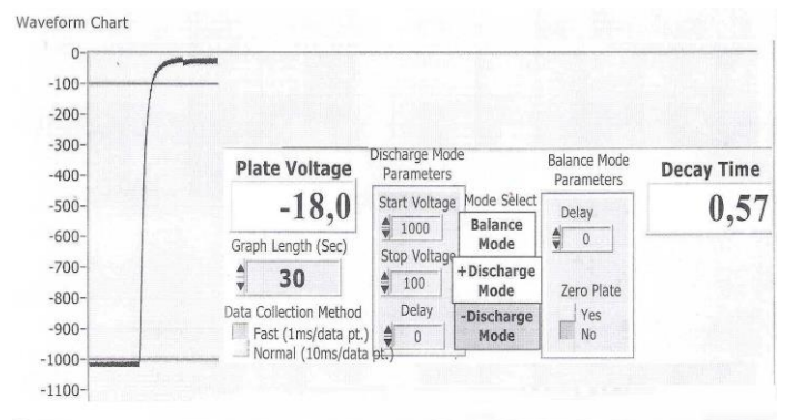
Decay time from - 1000V to -100V
