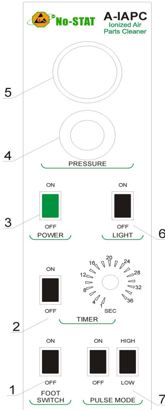
FIG. 2 VIEW OF THE CONTROL PANEL
